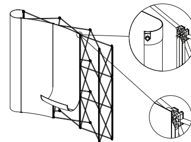
Attach panels in sequence to the mag bars starting at the top and smoothing down each side
